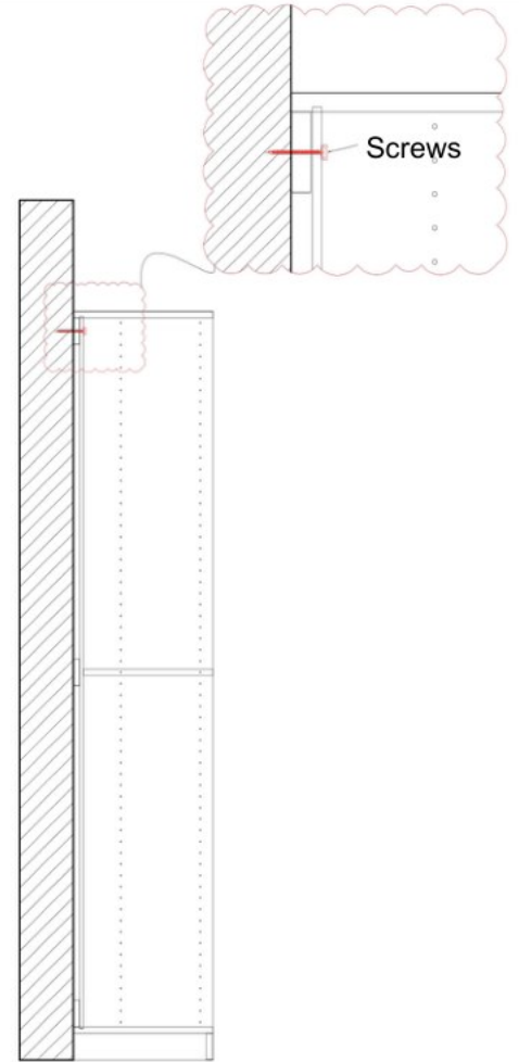
Section
